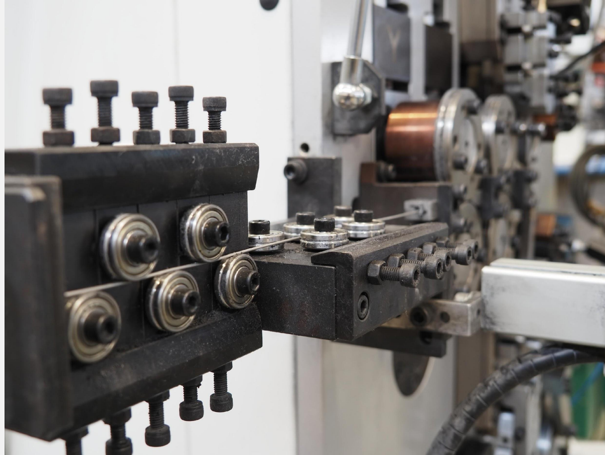
COILING MACHINES
